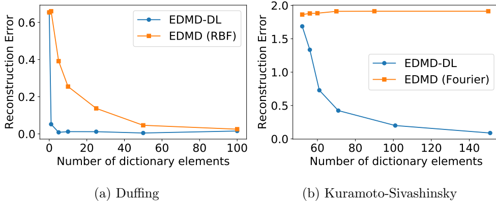
FIG. 4: Trajectory reconstruction error for EDMD-DL vs classical EDMD with hand-picked dictionary, whose sizes are varied. The errors are averaged over 50(10) random and unseen initial conditions for the Duffing (Kuramoto-Sivashinsky) system. We see that EDMD-DL requires much smaller dictionary sizes in order to capture the system’s dynamics.
