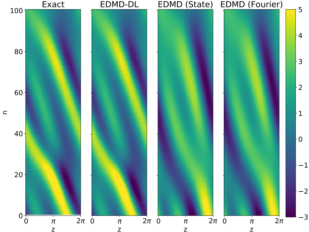
FIG. 8: Trajectory of the Kuramoto-Sivashinsky PDE reconstructed from Koopman decomposition using various algorithms. A random initial condition is picked from the same distribution as, but not from, the training data. We see that classical EDMD with both dictionaries cannot reproduce fine structures of the solution, whereas EDMD-DL performs well by adapting the dictionary to data. Also see Fig. 4 for a quantitative comparison of the reconstruction error vs number of dictionary functions.
