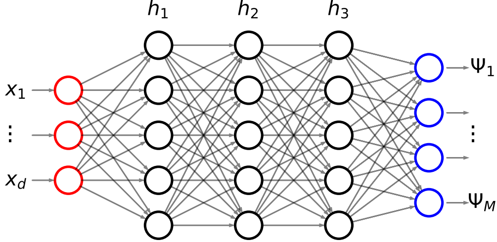
FIG. 1: Neural network function approximator for the trainable dictionary \Psi(x; \theta) . The network is fully connected and consists of 3 hidden layers h_1, h_2, h_3 . Arrows connecting layers corresponds to affine transformations followed by tanh activations. See Eq. (8).
