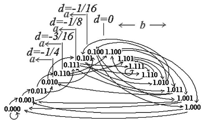
FIG. 5. Graphic presentation for the Bernoulli full shift and some dyadic misplacements.
