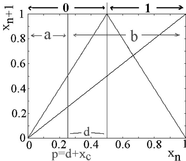
FIG. 1. Tent map and a misplaced partition at x = p .
