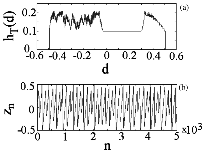
FIG. 4. (a) Topological entropy versus partition placement h_T(d) for experimentally collected chemical reaction [Belousov-Zhabotinsky (BZ)] data. (b) Time series of the data.
