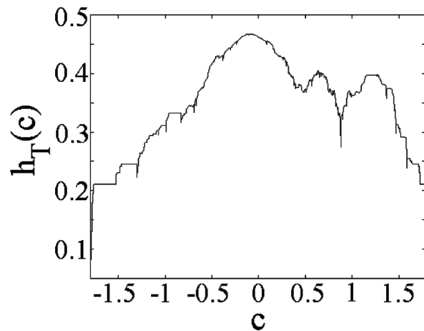
FIG. 3. For the standard Hénon map, the topological entropy h_T versus c , the parameter characterizing the misplaced partition at y = c . Features similar to those in Fig. 2 are seen.
