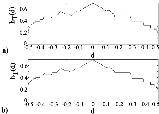
FIG. 2. For the tent map: (a) numerically computed h_T(d) function by following sequences of a chaotic orbit and (b) exactly computed entropy function h_T(d) .
