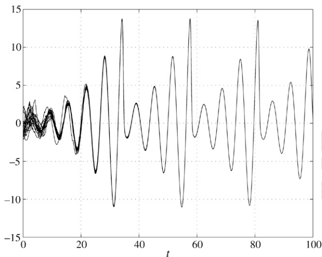
Fig. 5. Time evolution of the x_1 coordinate of the set of coupled Rössler oscillators using the moving neighborhood graph. Even though the neighborhood graph is instantaneously disconnected, fast switching allows for synchronization.
