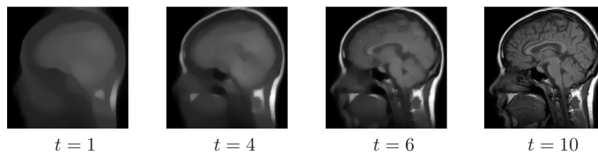
Figure 3. The images, U(t) = \int_0^t u(\cdot, s) ds , of the standard IDE (8) at t = 1, 4, 6, 10 . Here, \lambda(t) = 0.002 \times 2^t .
